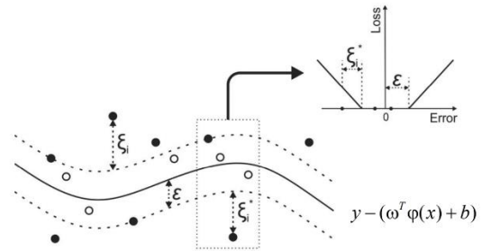
Figure 4: ε tube of nonlinear SVR
